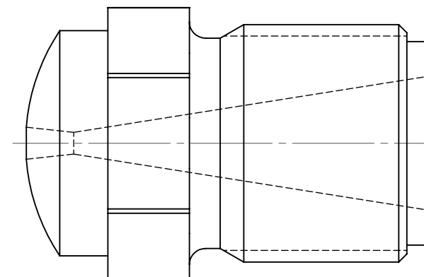
FULL INTERNAL TAPER DESIGN
