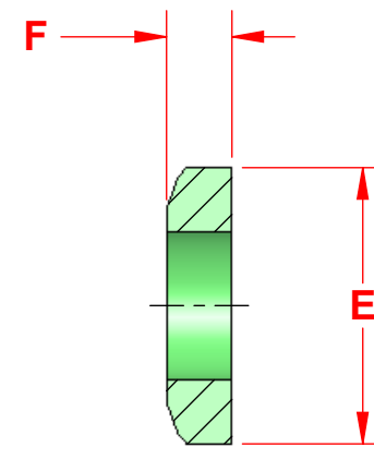
SECTION VIEW OF SEAT
